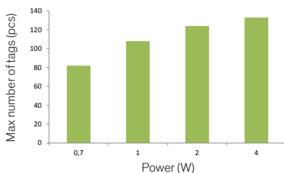
Stack test results (Scemtec SHL-2100)
